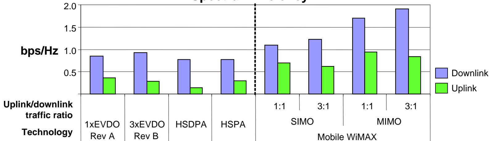
Spectral Efficiency
